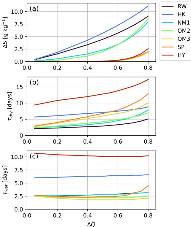
Figure 7. (a) Absolute value of the change in channel-averaged salinity \Delta S of different channels as a function of the change in discharge \Delta \tilde{Q} = \frac{Q_{\text{ref}} - Q_{\text{dry}}}{Q_{\text{ref}}} , where Q_{\text{ref}} is the yearly average discharge and Q_{\text{dry}} the decreased discharge. Note that \Delta S is independent of the sign of the change in discharge because absolute values are considered. (b) As (a), but for the response time \tau_{\text{dry}} due to a decrease in river discharge, i.e. a transition from Q_{\text{ref}} to Q_{\text{dry}} . (c) As (b), but for the response time \tau_{\text{wet}} due to an increase in river discharge, i.e. a transition from Q_{\text{dry}} to Q_{\text{ref}} .
