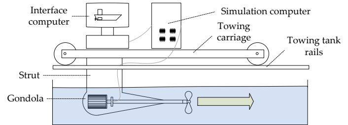
Fig. 3. General layout of a dynamic open water test. The computer on the left provides user interface and passes on set points to the simulation computer (also referred to as simulator). The simulation computer in turn simulates prime mover behaviour and controls the electric motor.
