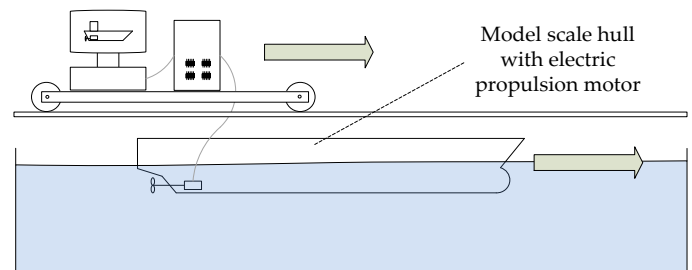
Fig. 4. General layout of a propulsion interaction test. The hardware on the towing carriage is the same as in the dynamic open water test.
