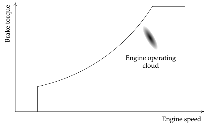
Fig. 5: Generic example of an engine operating cloud in the motor diagram. x and y axes can be modified to show different variables, such as fuel rack position instead of brake torque.
