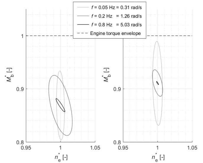
Fig. 6. Simulated engine operating clouds for ship (left) and model (right) described in Table 1, sailing in regular waves with different wave encounter frequencies. In this simulation, scale effects occur only on hull friction resistance and polar moment of inertia of the propulsion train. Brake torque, engine speed and wave frequencies are converted to full scale equivalents for ease of comparison.
