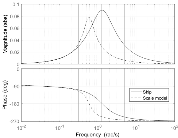
Fig. 7. Bode diagram of non-dimensional shaft speed response to non-dimensional wake fraction variations, \delta w^*/\delta n^* . Frequencies for the scale model have been corrected to full scale equivalents for ease of comparison. Verticals are drawn at frequencies of 0.31, 1.26 and 5.03 radians per second to facilitate comparison with Fig 6.
