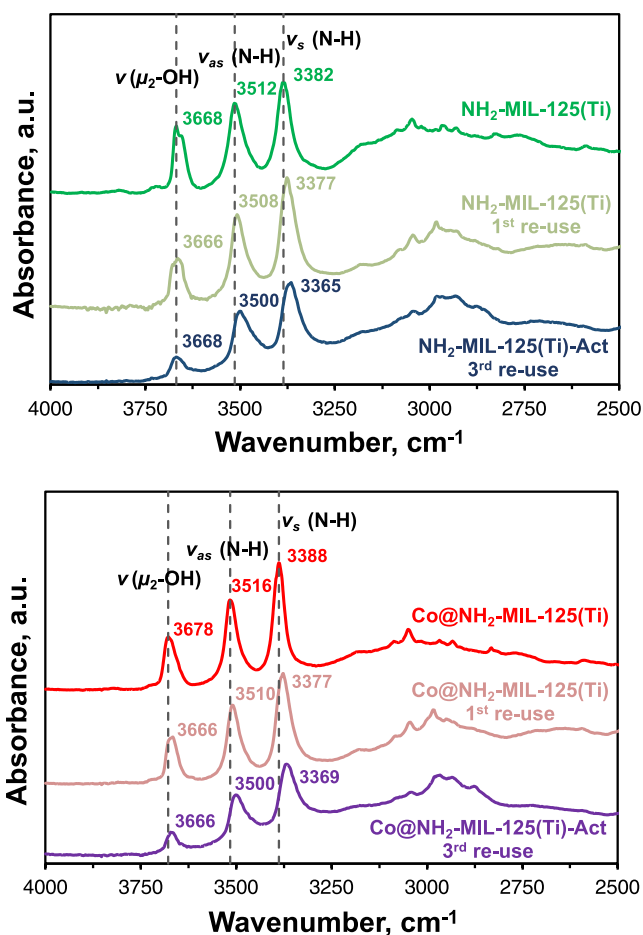
Figure 8. DRIFT spectra of (\text{Co@})\text{NH}_2\text{-MIL-125(Ti)} , preactivated, and reused photocatalysts.
