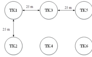
Figure 3: Layout of the gasoline tanks
