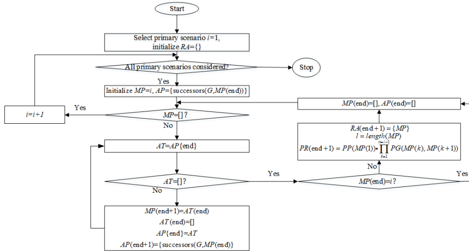
Figure 2: Algorithm flowchart for calculating all the possible paths and probabilities
