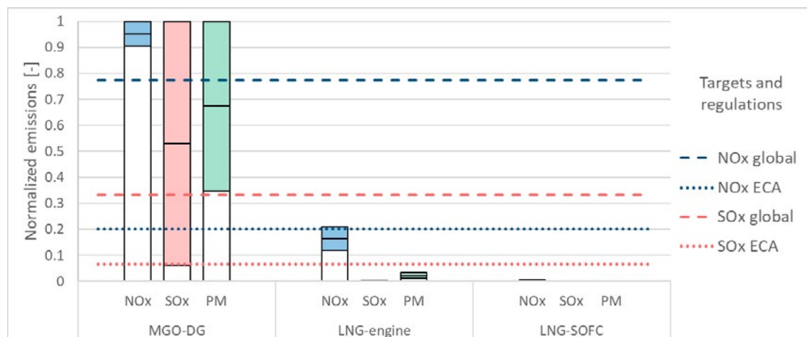
Figure 7.: NO_X , SO_X , and PM emissions from tank to wake.
