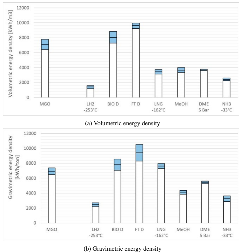
Figure 4.: Energy density of future fuels including the onboard storage system of the concerned fuel. The benchmark (MGO) has been compensated for the efficiency difference between diesel generators (43%) and SOFC (55%). The blue bars show the data ranges found in literature [68, 39, 6, 69], research projects, and supplier specifications and is based on LHV.
