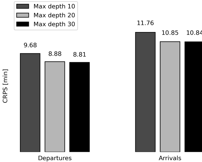
(b) CRPS values for delay prediction using varying values of the tree depth for RFR.
