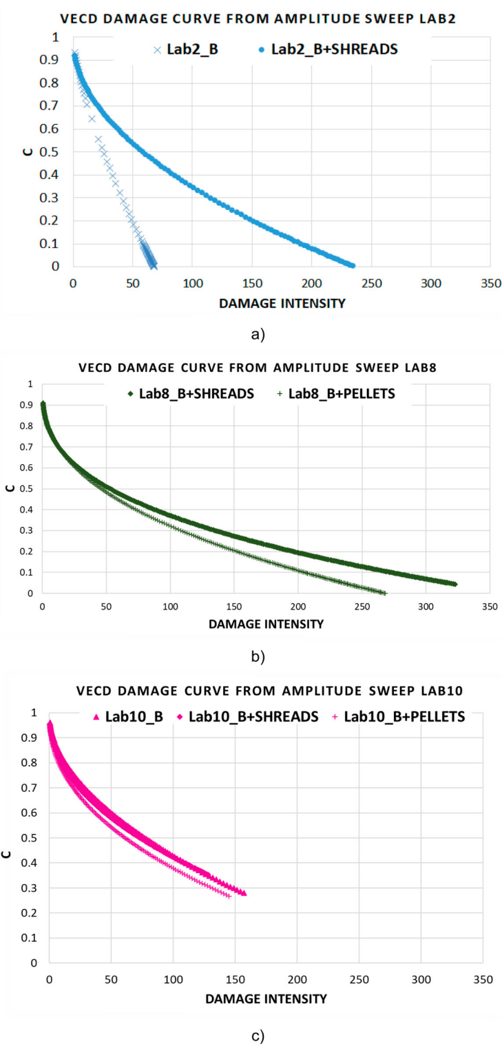
Figure 26. C-Damage Intensity: (a) Lab2, (b) Lab8 and (c) Lab10.
