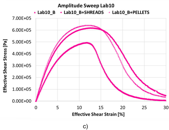
Figure 25. Plotting shear strain vs. shear stress: (a) Lab2, (b) Lab8 and (c) Lab10.
