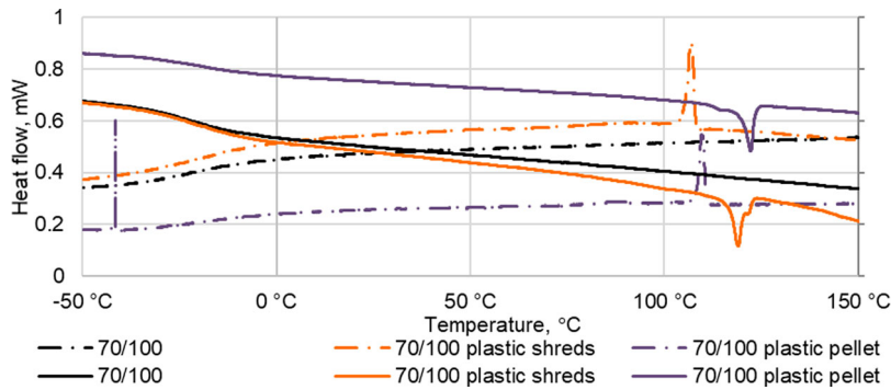
Figure 30. DSC on binders. The continuous lines are for the heating process and the dotted lines for cooling.
