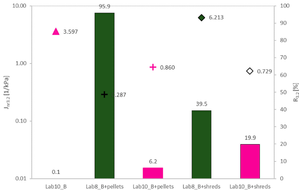
Figure 24. Strain recovery (% R ) and non-recoverable ( J_{nr} ) creep compliance at 3.2 kPa.
