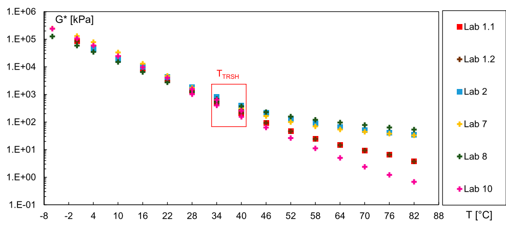
Figure 7. Modulus isochronal plot ( |G^*| vs. T ) at 1.59 Hz for B_{+pellets} .
