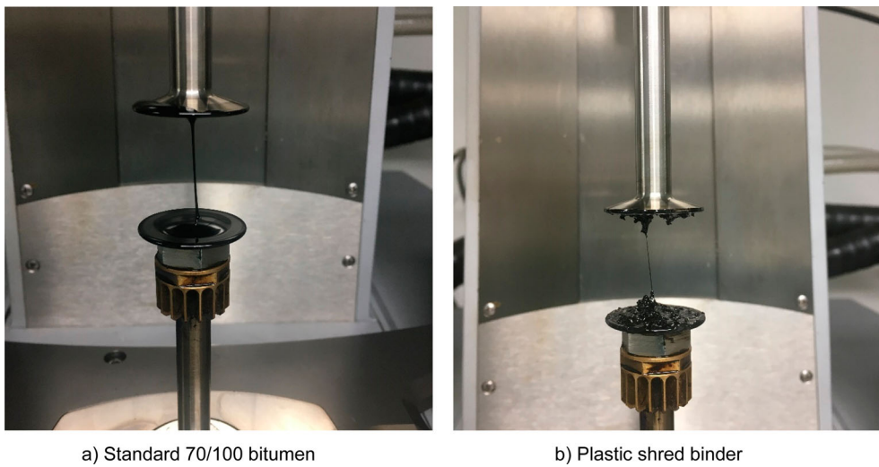
Figure 11. DSR sample at the end of the test with 25 mm plate and 100°C, for neat bitumen (a) and B_{+shreds} bitumen (b).
