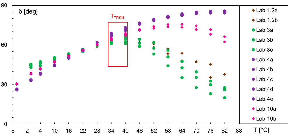
Figure 13. Evaluation of repeatability of Phase angle isochronal plot ( \delta vs. T ) at 1.59 Hz (10 rad/s) for Lab 1, 3, 4 and 10.
