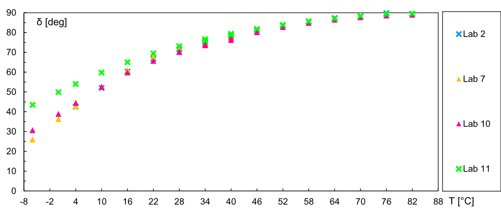
Figure 6. Phase angle isochronal plot ( \delta vs. T ) at 1.59 Hz for straight run binder B.
