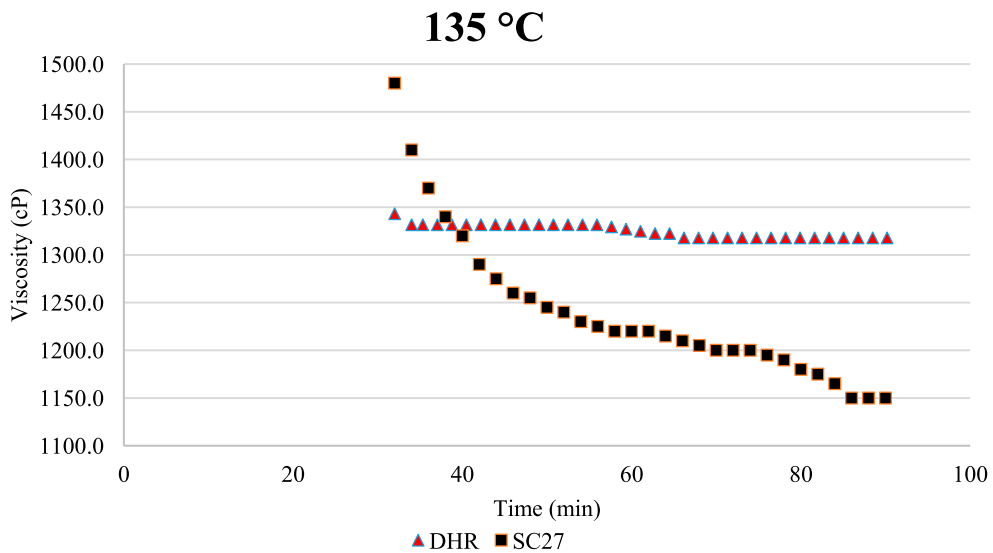
Figure 20. Viscosity measurements over time at 135°C and 100 rpm. Blend1 with shreds.
