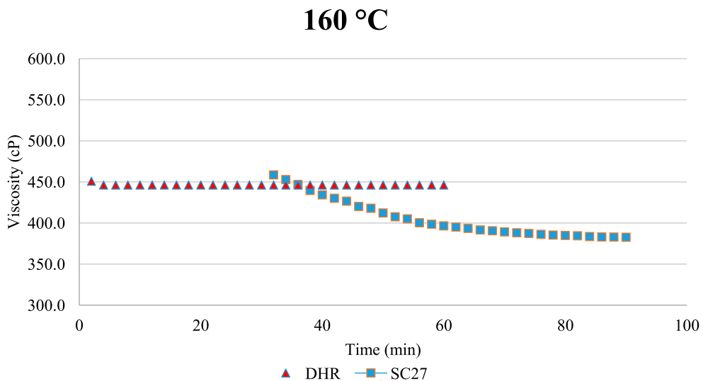
Figure 21. Viscosity measurements over time at 160°C and 100 rpm. Blend1 with shreds.
