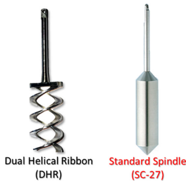
Figure 19. The dual helical ribbon (DHR) and the standard coaxial geometry (SC-27) were used in this study.
