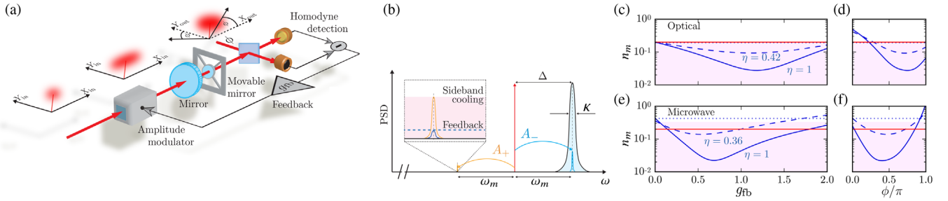
FIG. 1. (a) A cavity is driven by a coherent field with amplitude quadrature \hat{X}_{in} modified by an amplitude modulator fed with the output of the homodyne quadrature detection. The output field quadratures \hat{X}_{out} and \hat{Y}_{out} become correlated, depending on the homodyne phase \phi and on the nonresonant cavity driving at detuning \Delta . (b) The radiation pressure interaction in an optomechanical cavity with decay rate \kappa yields sidebands at mechanical frequencies \pm\omega_m , that correspond to processes which enhance ( A_+ , yellow) and reduce ( A_- , blue) mechanical energy. (c)–(f) Theoretical results for the phonon number of the cooled resonator at a low temperature (when standard sideband cooling is limited by backaction noise), as a function of the feedback gain amplitude g_{fb} (see [25]) [panels (c) and (e)] and the homodyne phase \phi [panels (d) and (f)], for the parameters of the experiment of Ref. [24] [panels (c) and (d)] and of Ref. [19] [panels (e) and (f)]. The light-pink areas indicate results beyond the backaction limit. Solid blue curves represent results for perfect detection efficiency \eta = 1 , dashed blue curves for \eta = 0.42 [27] in (c) and (d) and \eta = 0.36 [28] in (e) and (f), and finally dotted blue curves for no feedback. Red lines are the best up-to-date results obtained for systems operating at the quantum backaction limit, in the optical [24] (with standard sideband cooling) and microwave [19] (where squeezing is employed to improve the system performance) regimes.
