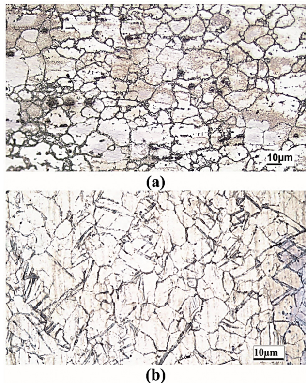
Fig. 1 – (a) The initial microstructure of the alloy after homogenization at 400 °C for 5 h and (b) the microstructure of the alloy after hot rolling at 430 °C.
