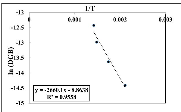
Fig. 9 – Variation of D_{GB} with reciprocal temperature.
