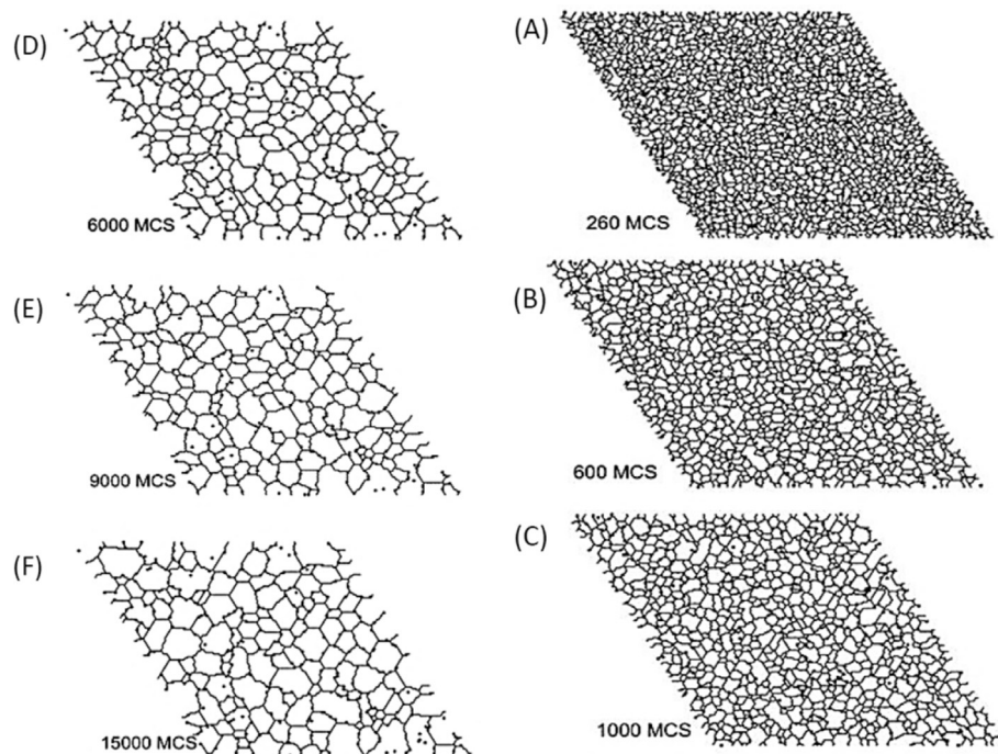
Fig. 5 – Monte Carlo prediction of the progressing as-annealed microstructure of AZ61 in the presence of 1.5% second-phase particles (indicated by black dots) at (a) 260, (b) 600, (c) 1,000, (d) 6,000, (e) 9,000, and (f) 15,000 MCSs.
