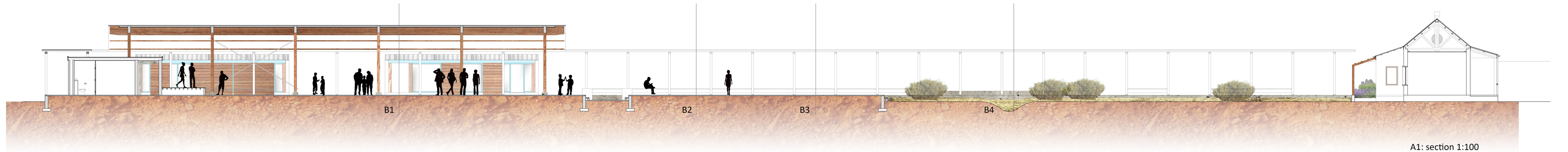
A1: section 1:100 Assembly hall / schoolyard / bioswale
