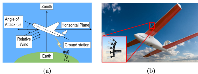
Fig. 1. (a) Angle of Attack (AoA) made by an aircraft. (b) Conceptual view of Hermes on a fixed-wing UAV.
