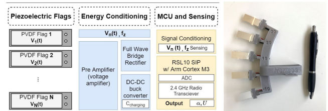
Fig. 11. Hermes system block diagram and fabricated sensor.
