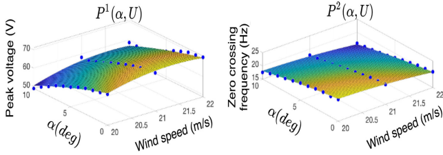
Fig. 12. Surface polynomials for expressing V_{pN} and f_{zN} as functions of \alpha and U .
