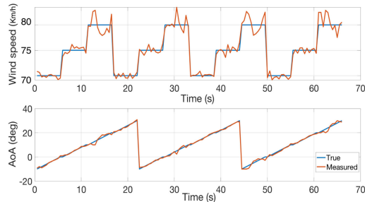
(a) Comparison between actual and estimated wind speed and AoA.
