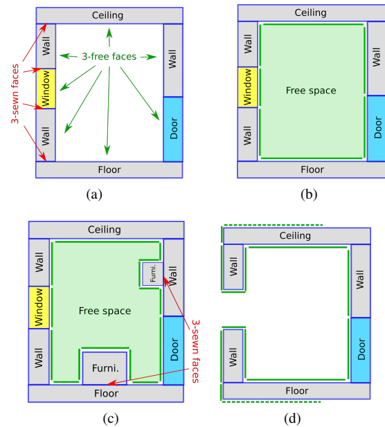
Figure 10: 2D projection of a free space volume reconstruction based on the approach of (Diakité et al., 2014a). (a) The faces that are not involved in a 3-sew operation among the model are detected. (b) Those faces are duplicated and 2-sewn between them to form a new volume corresponding to the free space. (c) The process works independently of the presence of other components in the scene. (d) In case of open window (or door), the free space volume cannot be closed.
