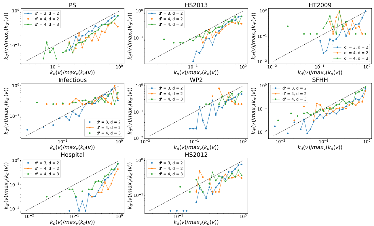
Figure 5. The d' -degree k_{d'}(v) versus the d -degree k_d(v) of a node v when (d', d) is equal to (3,2) (blue line), (4,2) (yellow line) and (4,3) (green line) respectively in each physical contact network. Each axis (e.g., k_d(v) ) has been normalized by its maximum (e.g., \max_v(k_d(v)) ). Only nodes whose d -degree and d' -degree are both non-zero are considered. The dashed line represent the reference case \frac{k_{d'}(v)}{\max_v(k_{d'}(v))} = \frac{k_d(v)}{\max_v(k_d(v))} . Note that both axes are presented in logarithmic scales. In total 30 logarithmic bins are split for horizontal axis.
