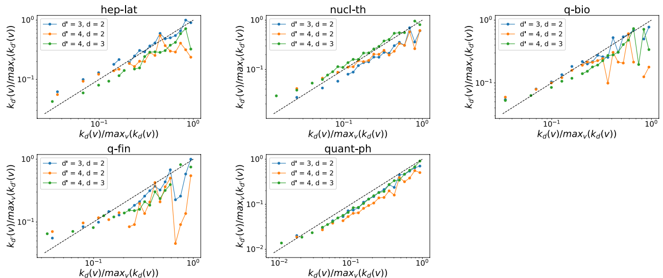
Figure 6. The d' -degree k_{d'}(v) versus the d -degree k_d(v) of a node v when (d', d) is equal to (3,2) (blue line), (4,2) (yellow line) and (4,3) (green line) respectively in each collaboration network. Each axis (e.g., k_d(v) ) has been normalized by its maximum (e.g., \max_v(k_d(v)) ). Only nodes whose d -degree and d' -degree are both non-zero are considered. The dashed line represent the reference case \frac{k_{d'}(v)}{\max_v(k_{d'}(v))} = \frac{k_d(v)}{\max_v(k_d(v))} . Note that both axes are presented in logarithmic scales. In total 30 logarithmic bins are split for horizontal axis.
