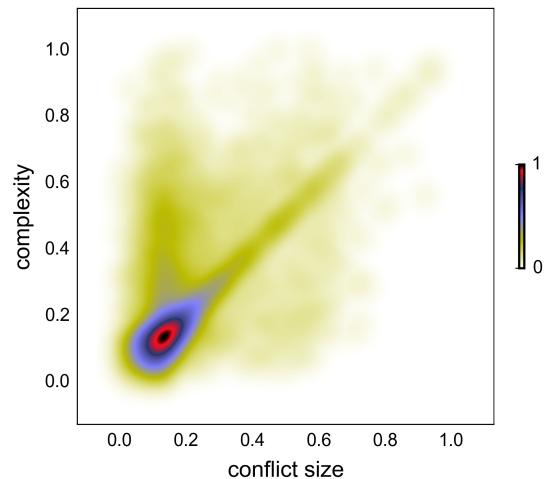
Figure 8. Density of conflicts plotted for conflict size and complexity. Single-ship conflicts are on the 45^\circ axis. The effect of the number of ships on complexity is chosen a = 0.5 .
