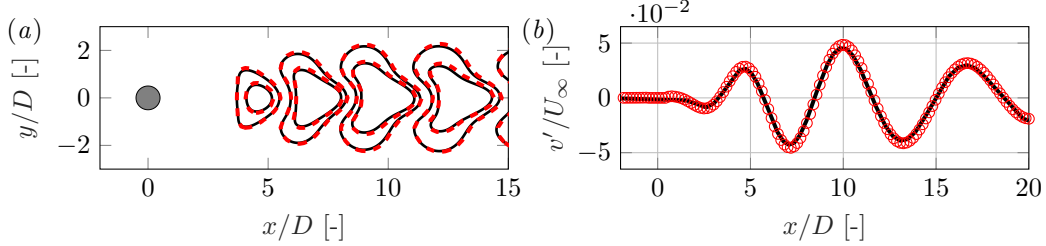
Figure 6: Dominant eigenmode ( v' ) when the base flow is unleashed, associated to \mu^c . (a) shows the xy -field, while (b) shows the profile along y = 0 . Solid black lines: q - \bar{q} from DNS, dashed red lines and red symbols: real part of global eigenfunctions from linear stability analysis.
