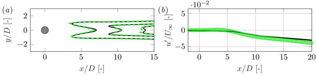
Figure 8: Dominant eigenmode of the flow ( u' ) when applying SFD, associated to \lambda^s . (a) shows the xy -field, while (b) shows the profile along y = 0 . Solid black lines: \mathbf{q} - \bar{\mathbf{q}} from DNS, dashed green lines and green symbols: real part of global eigenfunctions from linear stability analysis.
