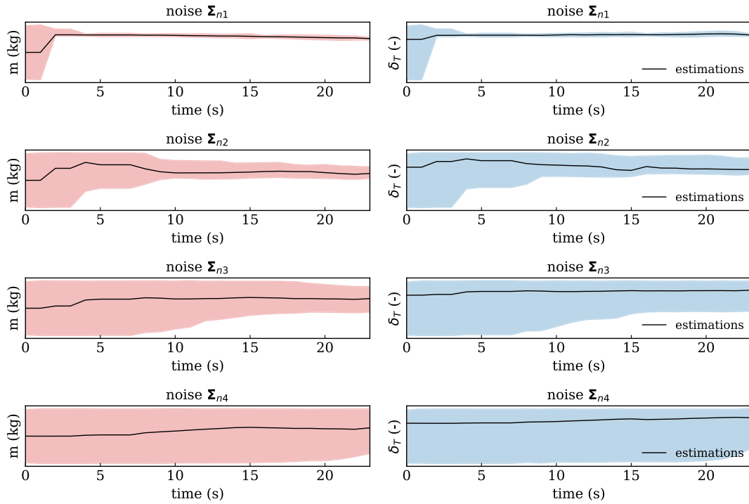
Fig. 7. Final distribution of m and \delta_T under different observation noise levels.
