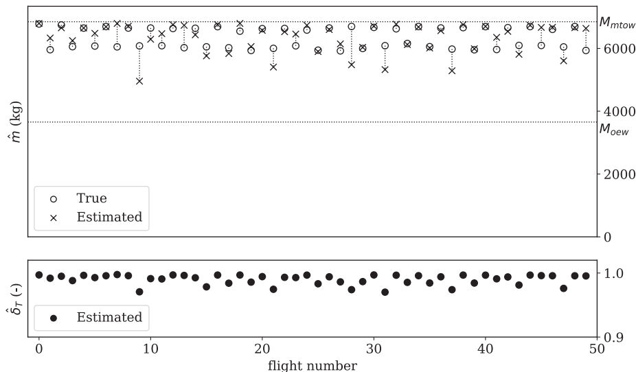
Fig. 8. Estimated results for all measurement flights.
