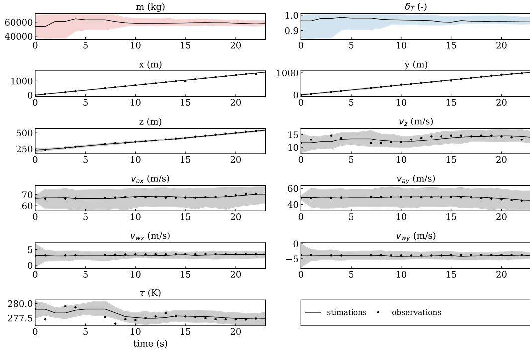
Fig. 6. Convergence of the particle filter states (noise level \Sigma_{n2} ).
