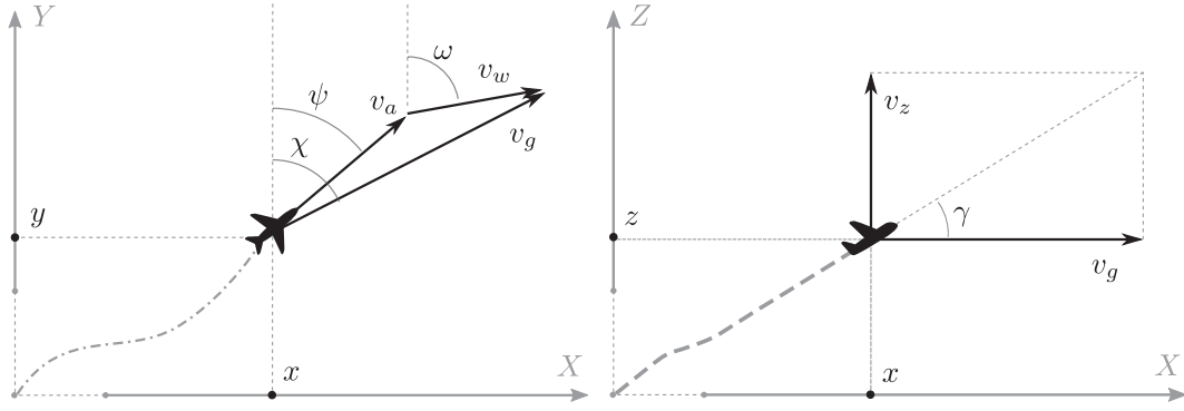
Fig. 1. Observed states in the flight dynamic system.
