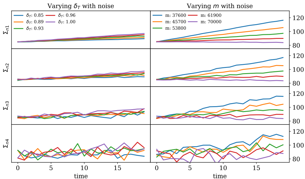
Fig. 13. Simulated speeds with different noise model.
