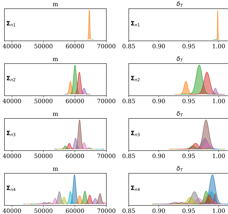
Fig. 14. Relationship between deviations in estimated thrust setting and mass.
