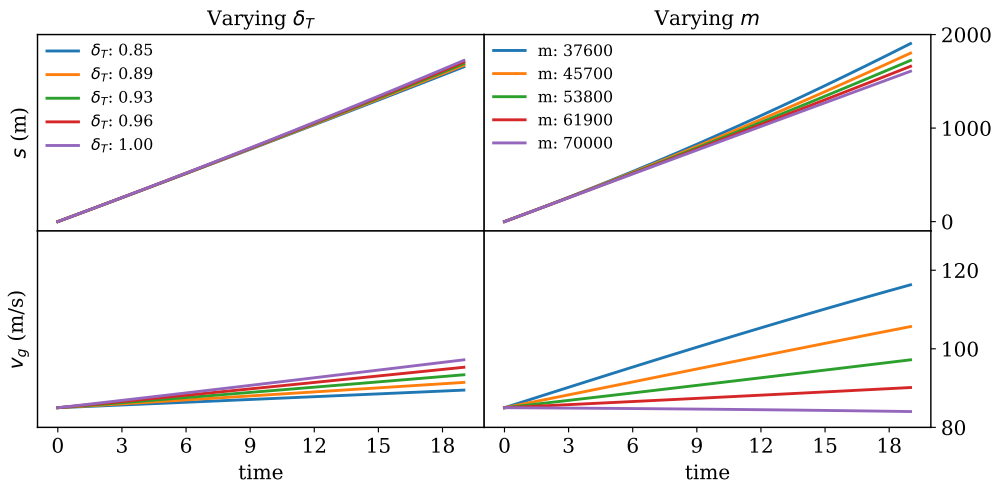
Fig. 12. Varying \delta_T versus varying m .
