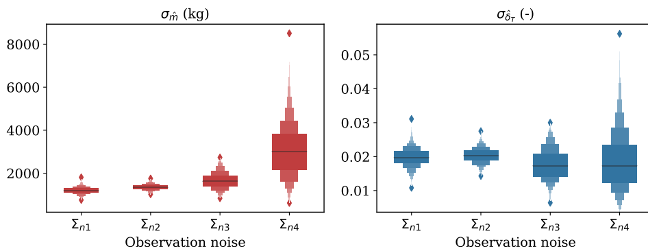
Fig. 11. Standard deviation of particles states on mass and thrust setting among 500 rounds of simulations under different observation noise models.
