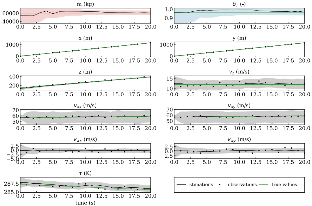
Fig. 4. Convergence of the particle filter states (noise level \Sigma_{n2} ).
