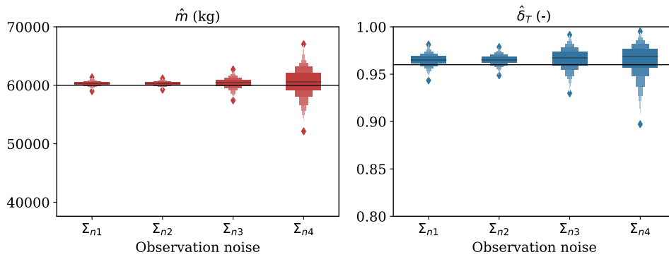
Fig. 10. The distributions of estimated mass and thrust setting based on 500 rounds of simulated trajectory under different observation noise models.
