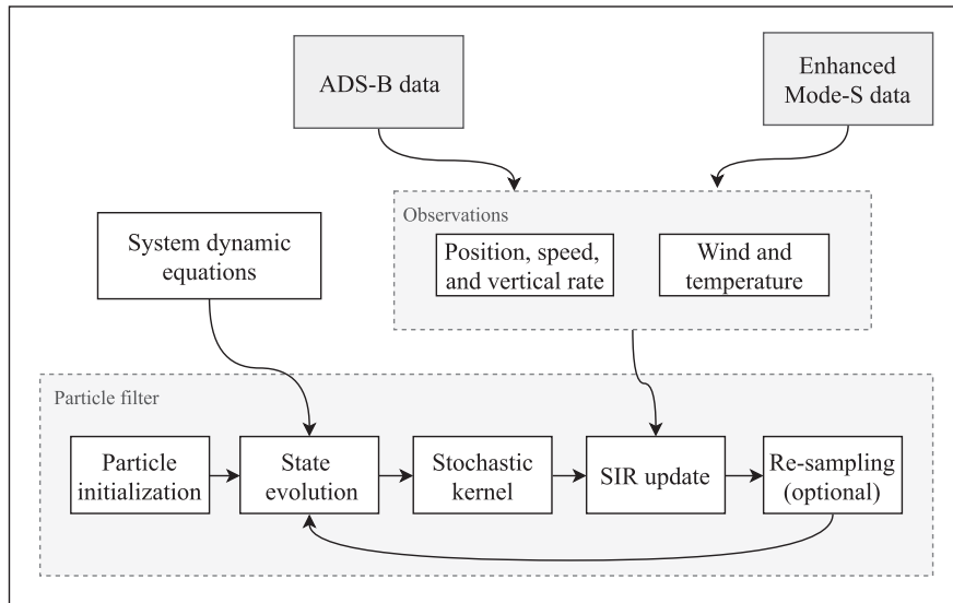
Fig. 2. Estimation diagram including the source of observations and process of SIR particle filter. Further details are given in Section 5.
