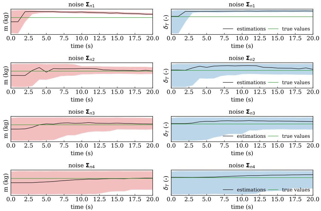
Fig. 5. Final distribution of m and \delta_T under different observation noise levels.
