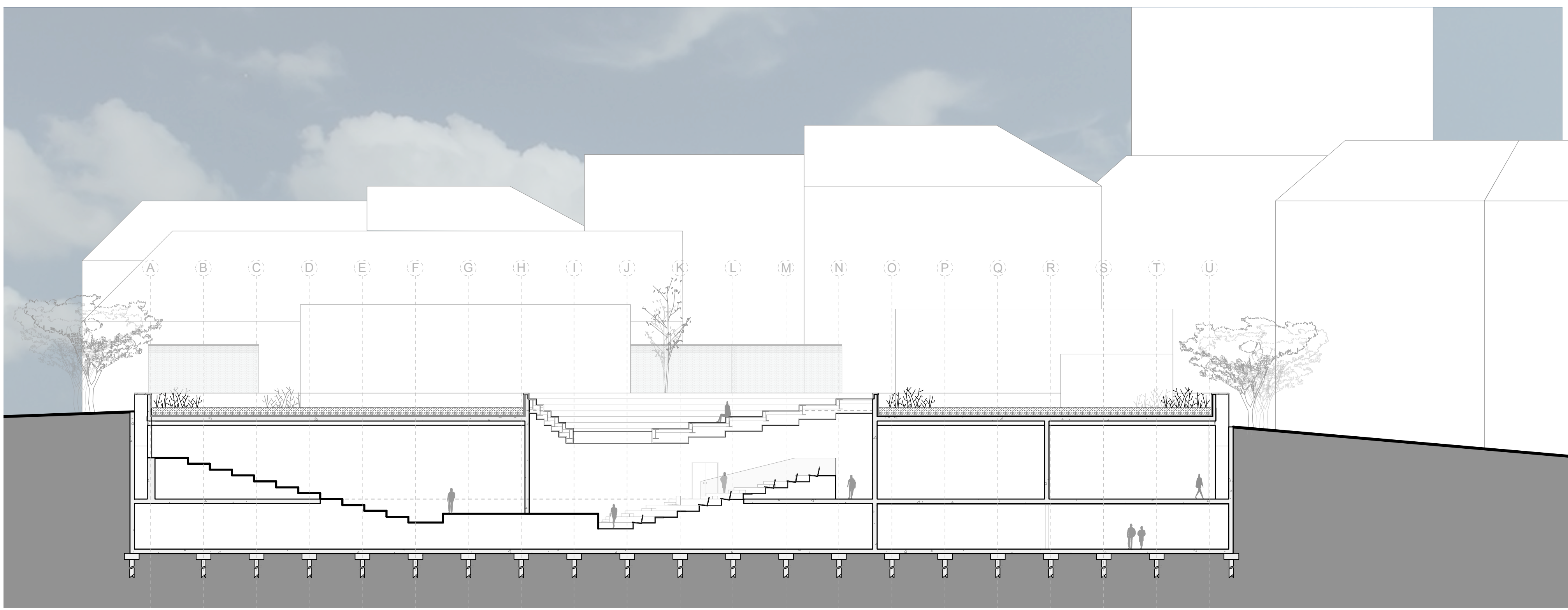
SECTION FF SCALE 1:200
