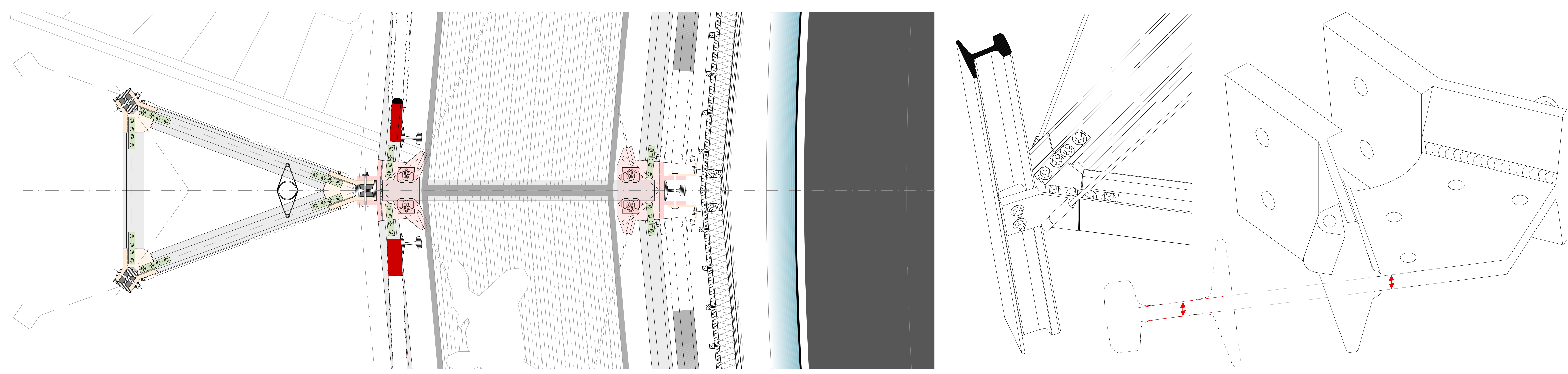
horizontal facade section with joints · 1:10
