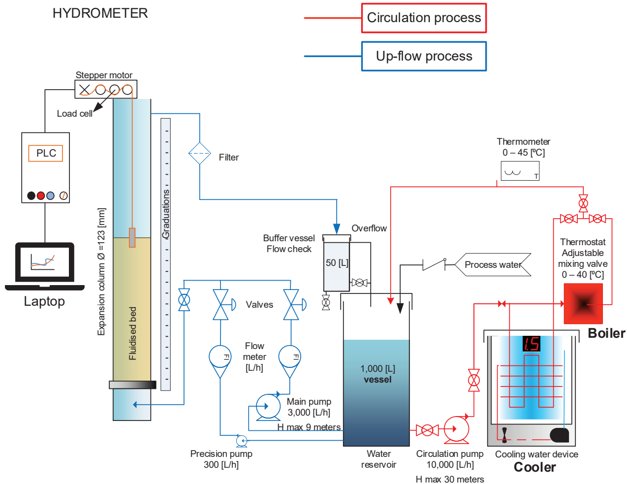
Figure 14 Schematic representation of the hydrometer experimental set-up
