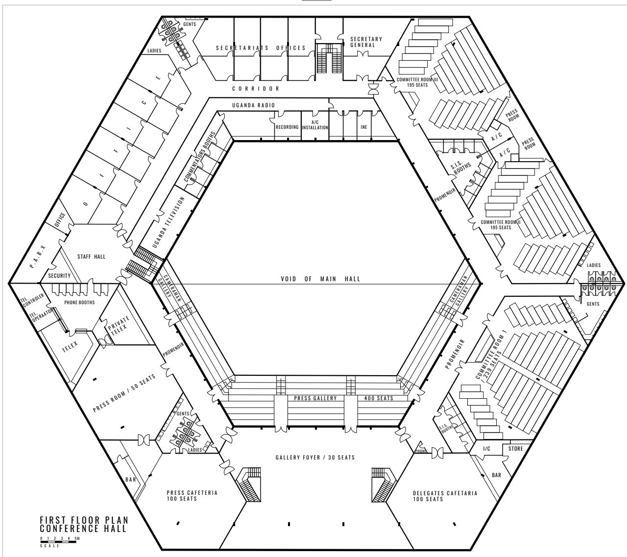
06 International Conference Centre, floorplan first floor, redrawn by author based on original scan. © Government of Uganda, 1971.
