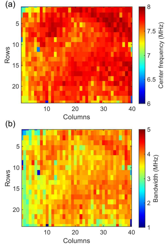
Fig. 6. (a) Center frequency. (b) Bandwidth \sim 6\ \text{dB} .
