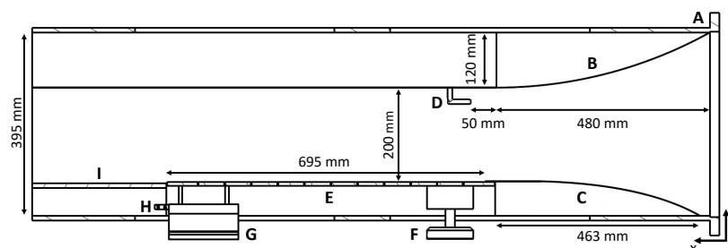
Figure 4. Schematic side view of direct force measurement setup for active dimples. A) Wind tunnel test section, B) Area reducing inlay, C) Area reducing ramp, D) Pitot tube, E) Active dimples model, F) Puck air bearing, G) Linear air bearing, H) Force sensor, and I) Rear flow guide. Flow from the right.
