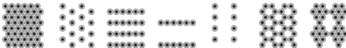
Figure 5. Dimple patterns 1-7. Note that this figure depicts the dimples as well as the outer rings where the adhesive can be applied, the inner circle indicates the dimple. Pattern numbering (1-7) from left to right and flow from below.
