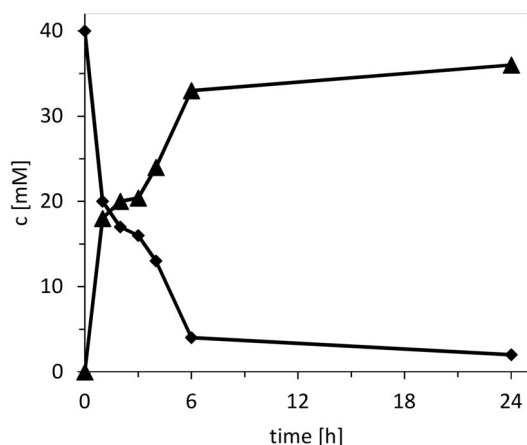
Figure 2. Time course of the chemoenzymatic etherification of 5-hexen-1-ol ( \blacklozenge ) into 2-(bromomethyl)tetrahydro-2H-pyran ( \blacktriangle ). General conditions: c(5\text{-hexen-1-ol}) = 40\text{ mM} ; c(\text{CVCPO}) = 100\text{ nM} ; c(\text{H}_2\text{O}_2) = 170\text{ mM} , c(\text{KBr}) = 160\text{ mM} ; 100 mM citrate buffer (pH 5); T = 25^\circ\text{C} .
