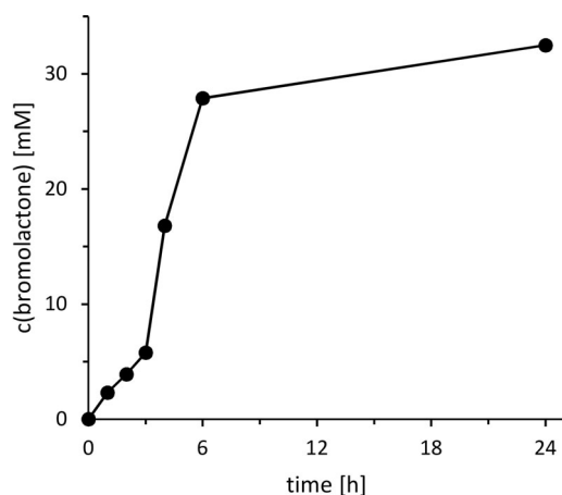
Figure 1. Representative time course of the chemoenzymatic bromolactonization of 4-pentenoic acid. General conditions: c(4-pentenoic acid)=40 mM; c(H 2 O 2 )=170 mM; c(KBr)=160 mM; 100 mM citrate buffer (pH 5); c(CIVCPO)=100 nM; T=25 °C.
