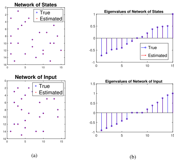
Fig. 1: Comparison of the true graph (blue circles) and estimated graph (red crosses) for both the states and input. (a) Adjacency matrices for the states graph (top) and the input graph (bottom). (b) Eigenvalues for both states and input graphs.
