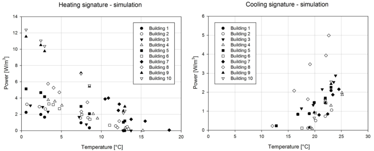
Fig. 2. Normalized energy signature data.
