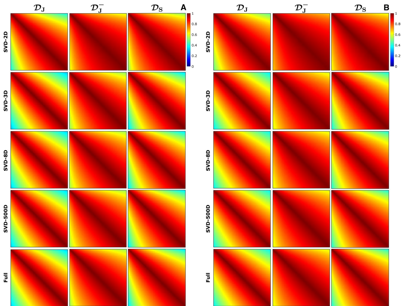
Fig. 5 Similarity maps derived from the SVD embeddings for different dimensionalities. The similarity matrices were calculated for a fixed T_2 = 80 ms, corresponding to WM ( A ), and for a fixed T_2 = 110 ms, corresponding to GM ( B ), using the Euclidean distance as a similarity measure. The diagonal elements of the similarity matrices are equal to one by definition. The horizontal and vertical axes of each similarity map represent the different possible T_1
