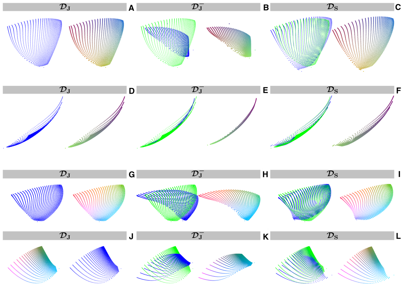
Fig. 2 Comparison of 2D and 3D embeddings for three different MRF flip angle patterns. Two-dimensional embeddings of \mathcal{D}_J (A,D), \mathcal{D}_J^- (B,E) and \mathcal{D}_S (C,F) produced by t-SNE (A–C) and SVD (D–F), respectively. The original embeddings (in blue) were registered to the corresponding embedding of \mathcal{D}_J (in green). These embeddings
