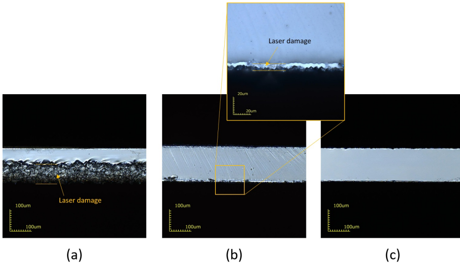
Figure 3.3: Cross-sectional views of wafer edges cut by different methods. (a) Laser and cleaving, resulting in a deep laser damage. (b) With TLS, the laser damage is limited to around 10\text{ }\mu\text{m} , as shown in the enlarged image. (c) 45^\circ cleaving without visible laser damage.
