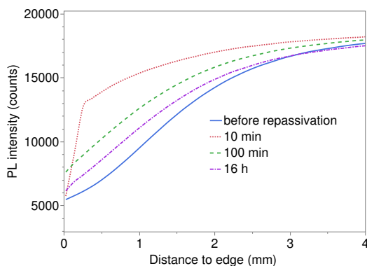
Figure 5.6: PL results of edge passivation over time, when the edge was exposed in the air.
