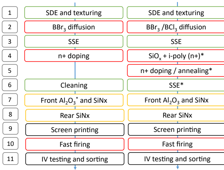
Figure 2.7: Typical process flows of n-PERT (left) and i-TOPCon (right) cells. Wet chemical processes are in green, high temperature processes are in red, vacuum processes are in yellow, and other processes are in black.*Different processes were reported by different companies or institutes.
