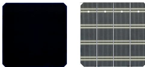
Figure 5.1: Images of a solar cell fabricated for edge passivation evaluation. The left image is the front side of a cell. The right image is the rear side of a cell, and the cell was cut into 1/4 sizes through the gaps.
