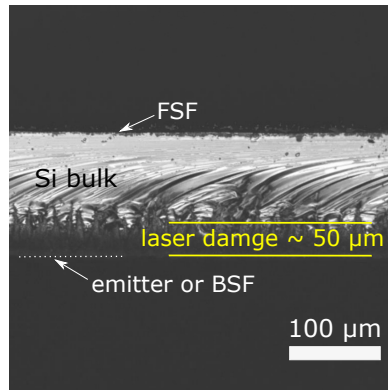
Figure 4.5: Cross-section of the laser cutting area
