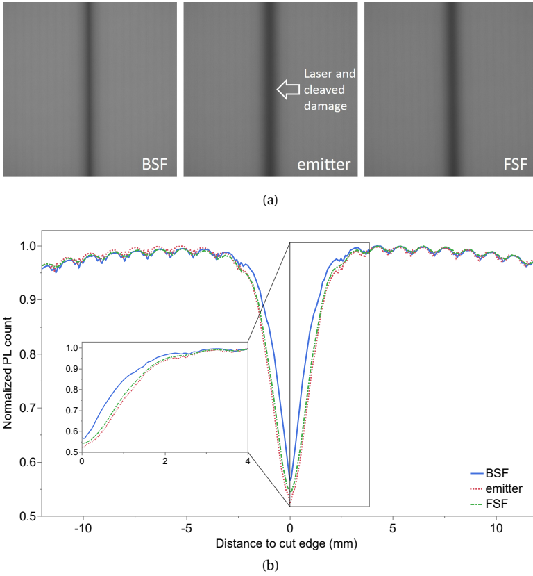
Figure 4.7: (a) Photoluminescence images of the laser-cut regions after laser cut and cleaving, with the same scaling. From left to right: BSF, emitter and FSF. (b) Cross-section of PL profiles from the cell edge.
