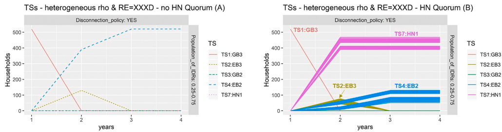
Fig. 5. TSs when households had heterogeneous discount rates, under the disconnection policy.
