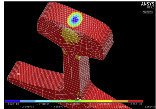
Fig. 8. Static contact solution.
