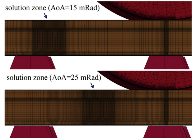
Fig. 5. Remesh rail model to adjust the position of solution zone.
