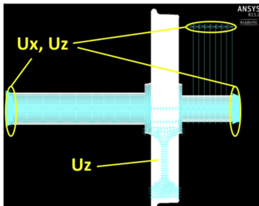
Fig. 7. Displacement constraints.
