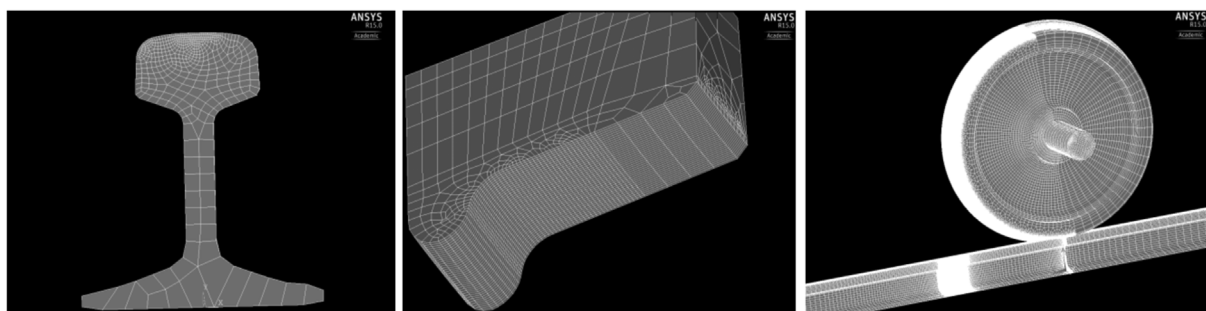
Fig. 4. Wheel and rail meshes. (a) Mesh of rail cross section (b) Mesh of wheel tread (c) Overview of wheel & rail meshes.
