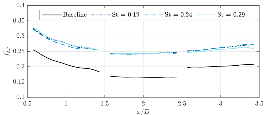
Figure 11. Average available power \overline{f_{AP}} in the wake of a turbine operated with DIC compared to baseline operation. The \overline{f_{AP}} is based on cross-sections of the measured streamwise velocity field.
