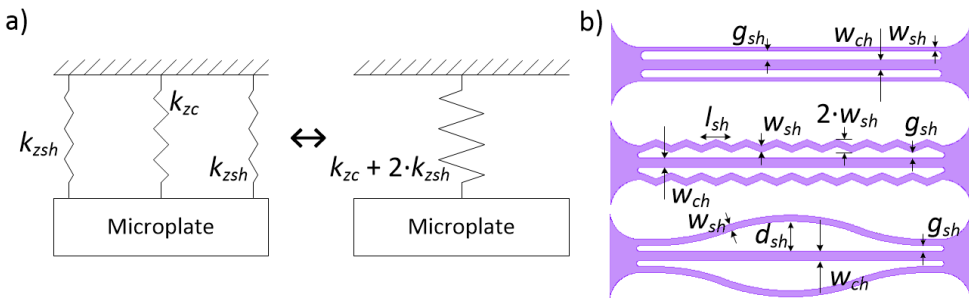
Figure 2.16: Side hinges: (a) Influence of the side hinge on the vertical spring constant (b) Geometry of side hinges which should provide larger k_z .
