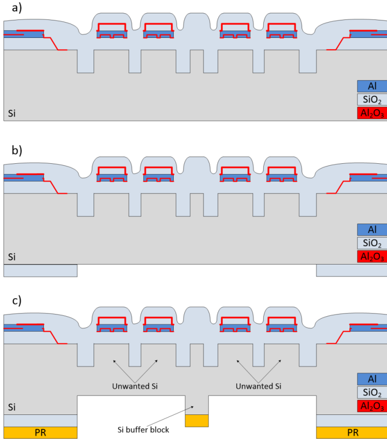
Figure 4.8: Main steps for hinges fabrication: (a) Front side hinge definition and stop layer deposition; (b) The backside hard mask definition (c) The first backside DRIE etching step.
