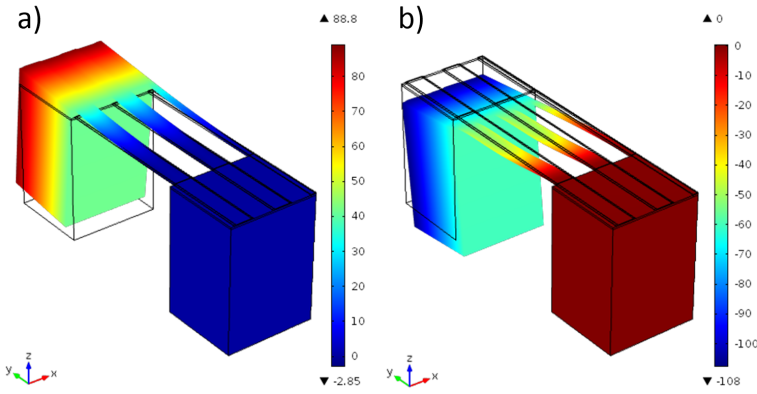
Figure 2.34: (a) Simulation results for N_a = 4 and l_y = 800 \mu\text{m} : (a) initial microplate position due to pre-stress and (b) final microplate position at 420 \text{ }^\circ\text{C} . (Only one half of the system is simulated to save computational time).
