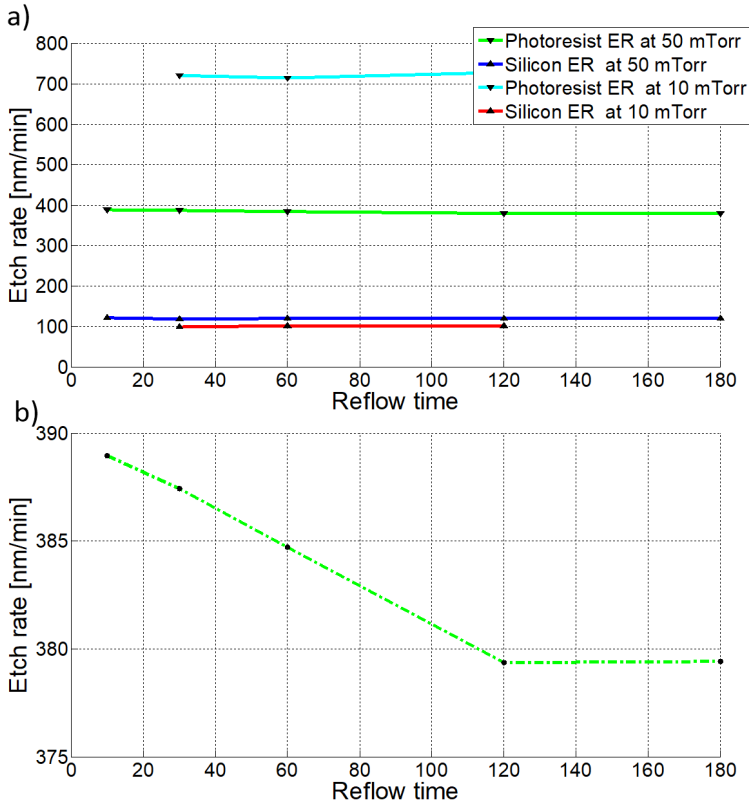
Figure 3.9: (a) Photoresist and Si etch rates versus resist reflow time at 10 mTorr and 50 mTorr; (b) zoom in on the photoresist etch rate at 50 mTorr.
