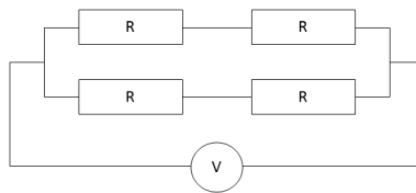
Figure 2.30: Electrical schematics of heater connections on each side of the actuator system.
