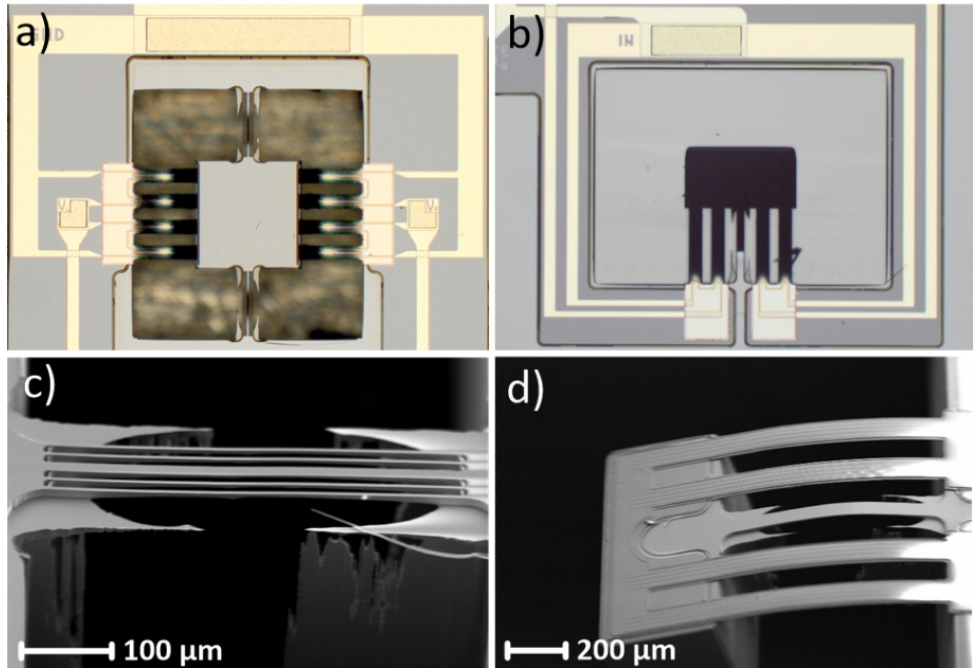
Figure 4.12: The released actuators: Optical images of MEMS actuator system for (a) x direction scanner and (b) y direction scanner. SEM images of (c) torsional and (d) deflective hinge.
