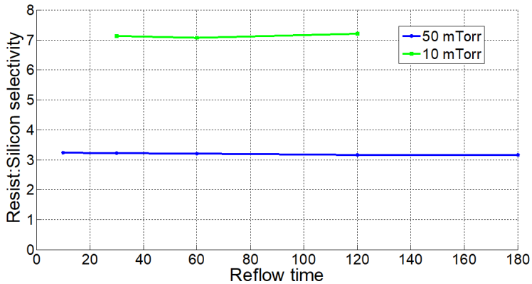
Figure 3.10: The Photoresist to Si etching selectivity at 10 mTorr and 50 mTorr.
