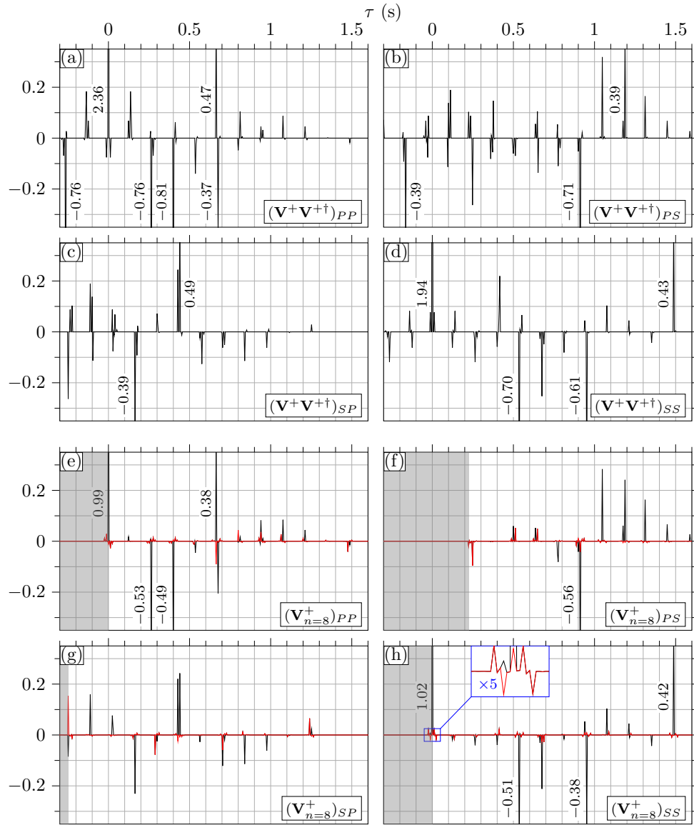
Figure 6. Idem as Figure 5 but associated with the model Elastic #2 (see Figure 2). In this case, the dereverberation operator has acausal events on the diagonals ( PP and SS components) due to so-called fast multiples (these are multiples that share a temporal overlap with the forward-scattered events, for details see Reinicke et al., 2018). The acausal events on the diagonals appear to be an issue for the Wilson algorithm. The dereverberation operator is reconstructed only up to a relative error in the order of 10 % (see Figure 4), instead of numerical noise as in the previous example in Figure 5.
