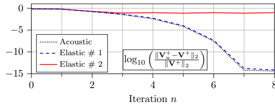
Figure 4. Convergence of the 1D-scalar and 2D-matrix Wilson algorithms in Eqs. 10 and 30 associated with the dereverberation operators ( V^+ and \mathbf{V}^+ ) of the acoustic and elastic models in Figure 2, respectively. The convergence is defined as the relative error with respect to the true solution as indicated by the legend. For the acoustic and the Elastic #1 case, the Wilson algorithm converges up to numerical noise within seven iterations. For the Elastic #2 case, the relative error converges to approximately 10 %.
