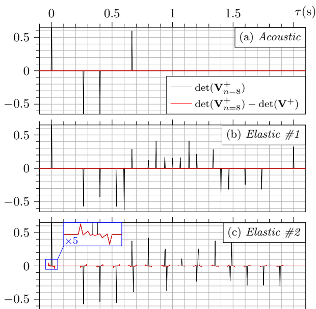
Figure 7. Determinants of the retrieved dereverberation operators (black) and the difference with respect to the modeled solutions (red). The panels are associated with the (a) Acoustic , (b) Elastic #1 , and (c) Elastic #2 , cases shown in Figures 3, 5 and 6, respectively. In the Acoustic case, the dereverberation operator is a scalar function, and hence, identical to its determinant. Nonetheless, it is shown for completeness. For the Elastic #2 case, the determinant of the retrieved dereverberation operator is not minimum-phase, which can be easily seen via the acausal events shown in the magnified box in blue. The difference plot indicates that acausal events are absent in the determinant of the true solution, which possesses a minimum-phase property.
