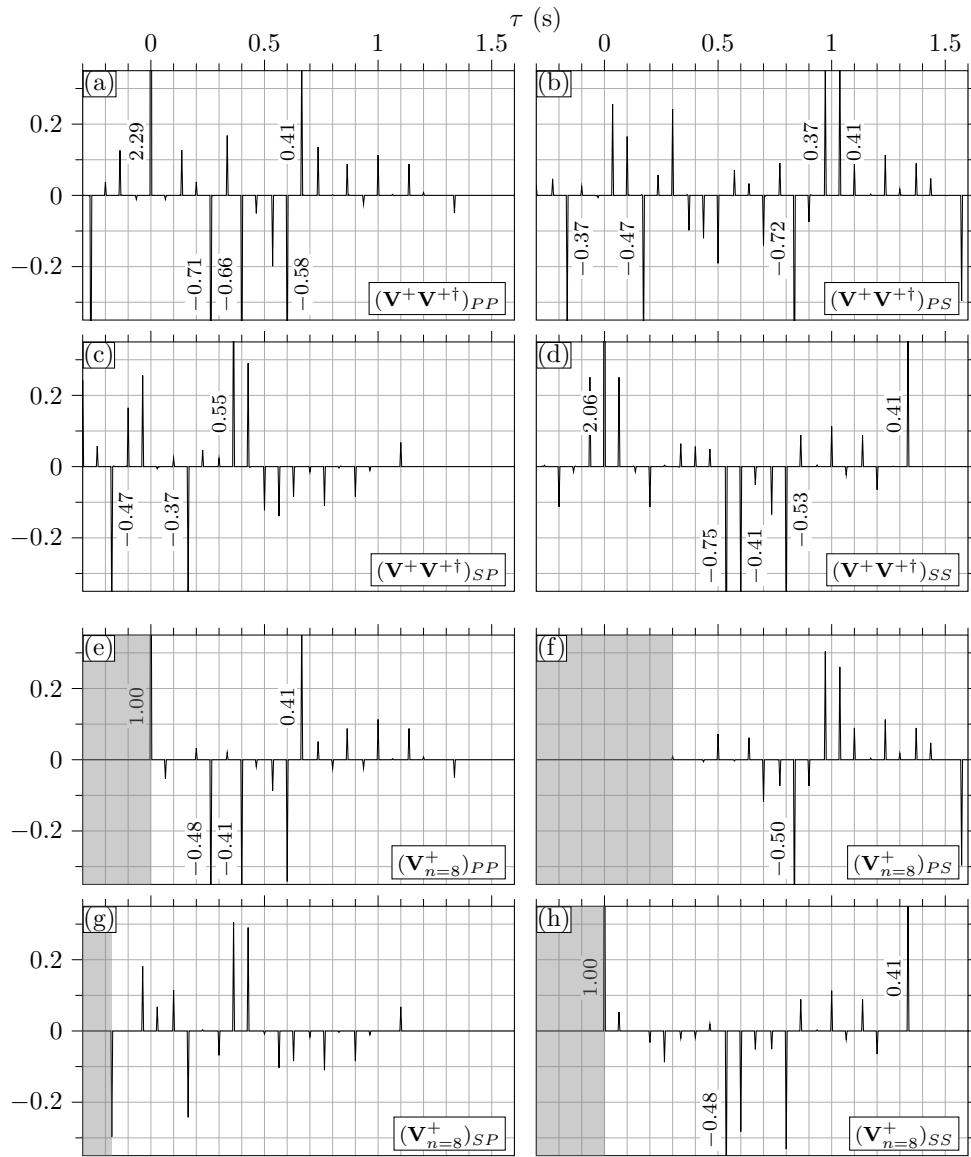
Figure 5. (a)-(d) Normal product \bar{\mathbf{V}}^+ \mathbf{V}^{+\dagger} of the dereverberation operator associated with the model Elastic #1 (see Figure 2). The panels show the four elastic components analogously to the 2 \times 2 matrix in Eq. 17. (e)-(h) Retrieved dereverberation operator after eight iterations. The grey areas indicate the time samples that are muted by the modified operator \bar{\mathbf{\Theta}}[\cdot] in Eq. 30. We do not show a difference or reference plot because the retrieved and modeled dereverberation operators are identical up to numerical noise (see convergence in Figure 4). All panels show responses in the time domain to facilitate the interpretation.
