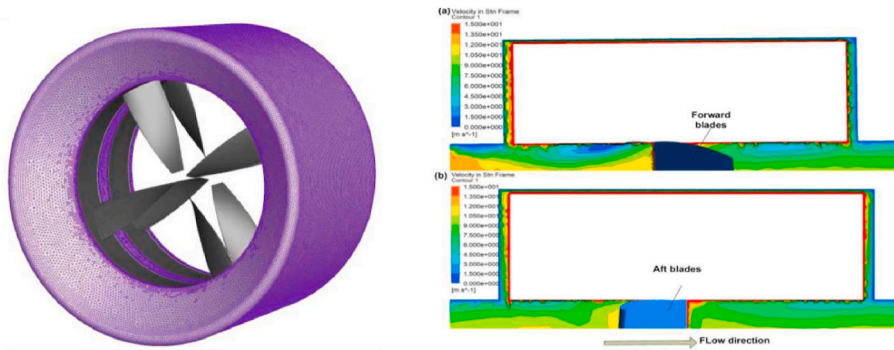
Fig. 24. Mesh division and gap fluid velocity distribution of the rim-driven thruster [209].
