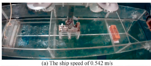
Fig. 11. Experiment of the bubble morphology at two different ship speeds [101].
