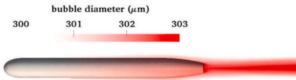
Fig. 12. Bubble diameter distribution analysis [104].
