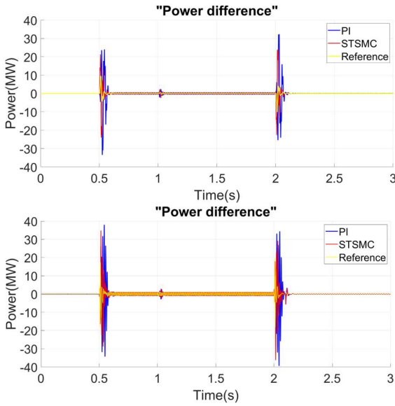
Fig. 9. Power difference using PI controller and STSMC: (a) in upper and lower leg in arm of each phase (b) between two legs
