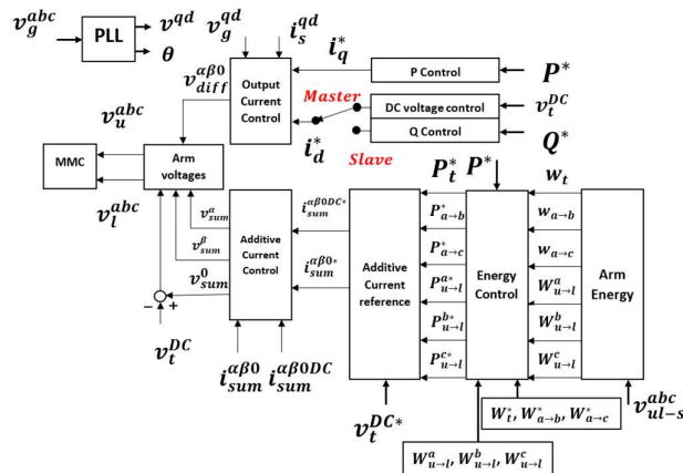
At the bottom, the circulating current (CC) and energy balancing control are presented. At the top-left, a phase-locked loop (PLL) is presented that can estimate an angle between grid voltage and point of common connection (PCC) for control loops.
