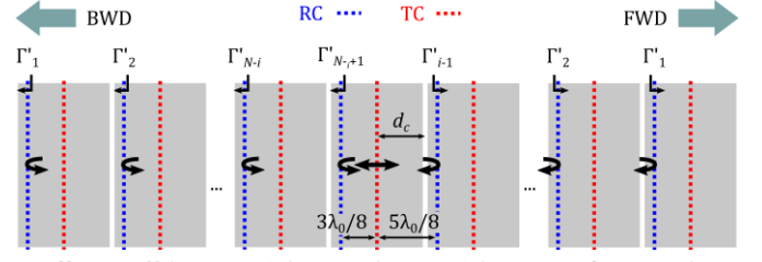
Fig. 5. Schematic of a transducer where each grey rectangle corresponds to a unit cell with marked RC and TC. For the i^{\text{th}} unit cell, the directionality can be calculated by considering its TC and all the RCs at both sides.
