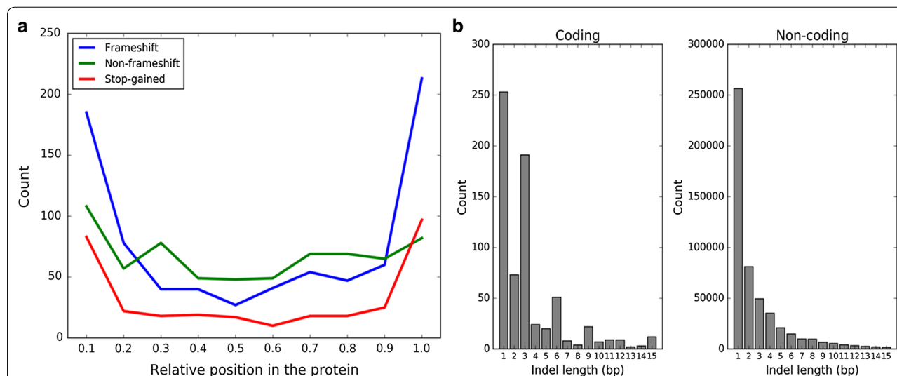
Fig. 3 a Relative position of frameshift, non-frameshift indels, and stop-gained variants. Frameshift variants are enriched in N- and C-terminal parts of the protein. Frameshift variants at the N-terminal sites are potentially “rescued” by alternate start-codons. Frameshift variants at the C terminal end are likely not disruptive since a functional protein might still be translated. b Distribution of lengths of coding and non-coding indels. In-frame indels (i.e. indels with lengths of 3, 6, and 9 nucleotides) are enriched in coding regions
