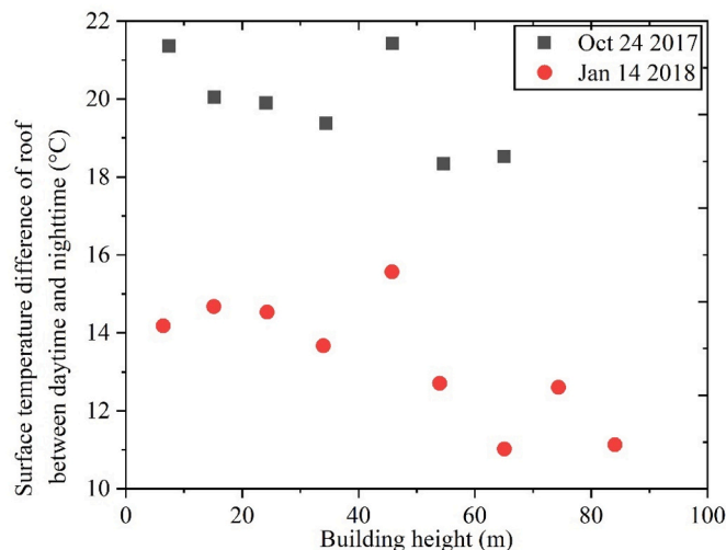
Fig. 13. Difference between daytime and night in roof temperature vs. building height.
