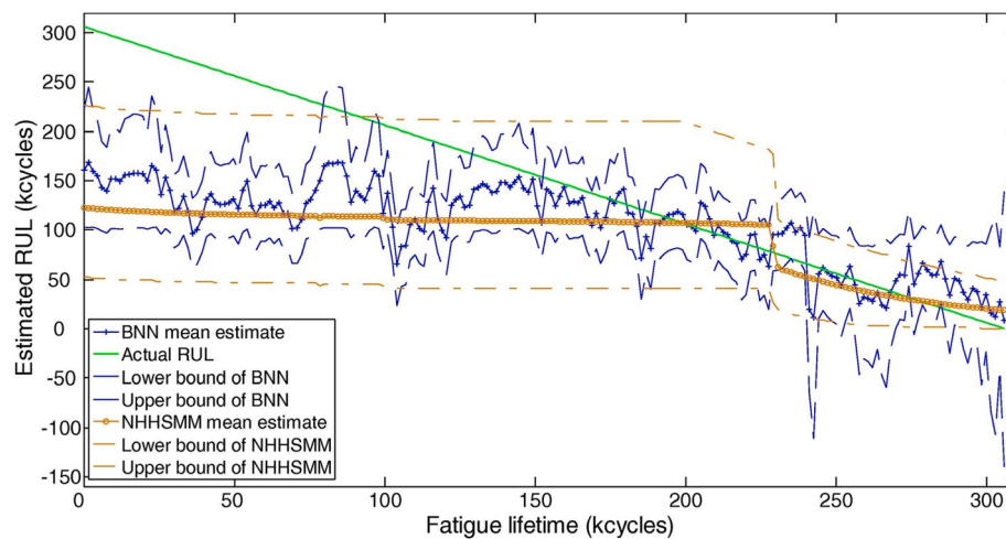
Fig. 8. RUL prognostic results for an OHT carbon/epoxy coupon using BNN and NHHSM methods (lower and upper bounds shown for both models represent 90% confidence intervals) [134].
