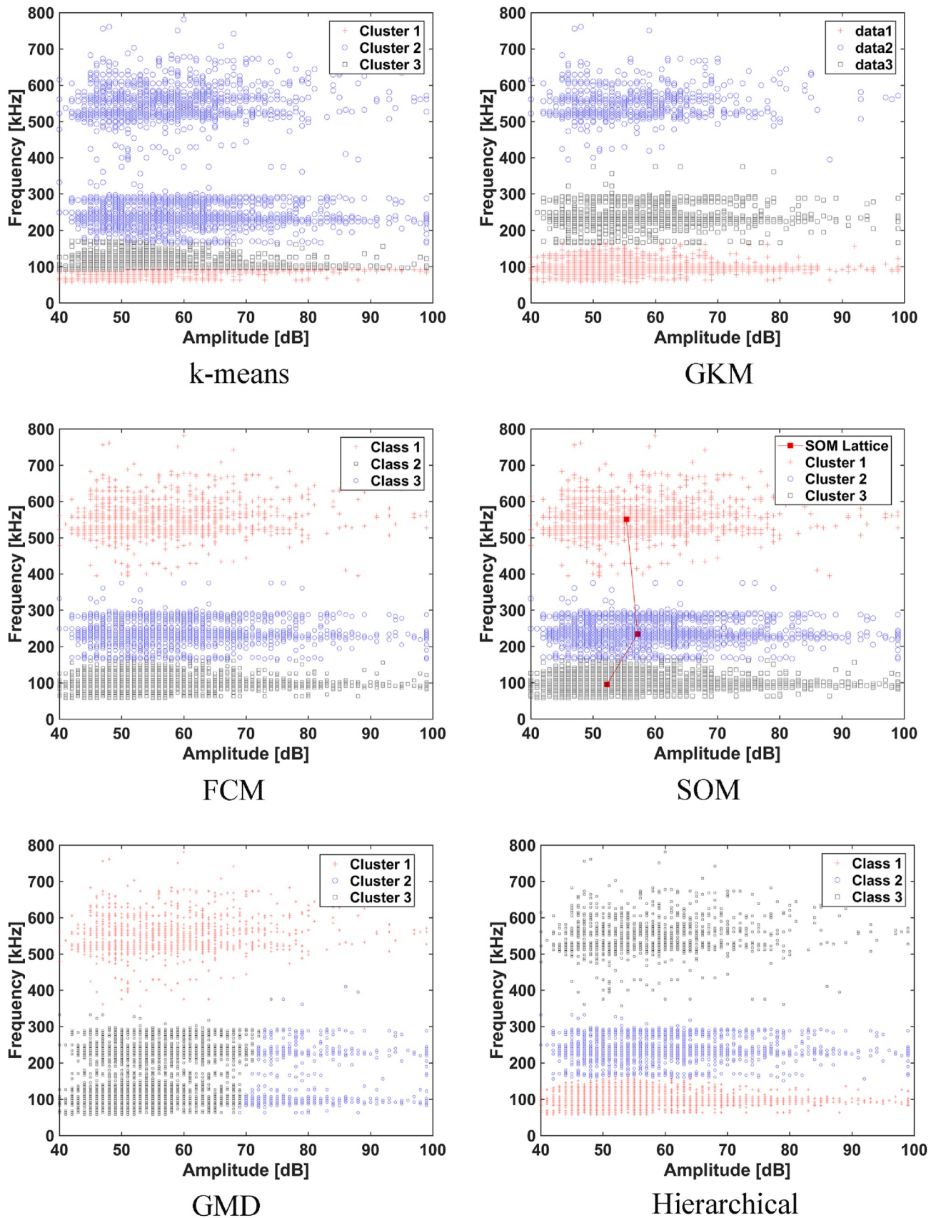
Fig. 5. The performance of k-means, GKM, FCM, SOM, GMD and hierarchical methods to partition the AE signals into three groups (the data belongs to carbon/epoxy laminates subjected to the indentation load) [5].
