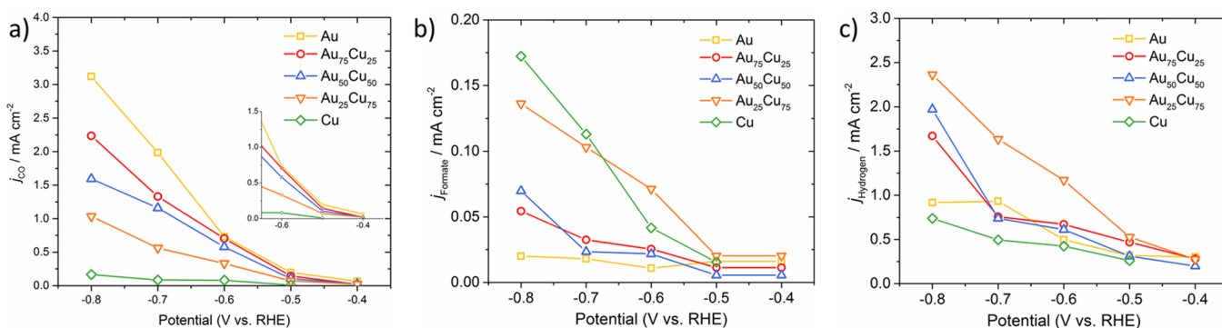
Figure 9. Activity of bimetallic catalysts for two-electron products. Partial current densities of (a) CO, (b) \text{HCOO}^- , and (c) \text{H}_2 are shown as a function of applied potentials. Inset: a zoom-in image of the potential region of -0.4 to -0.6 V vs RHE.
