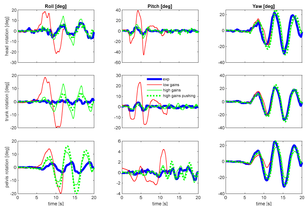
Figure 2. Slalom validation for body rotation. Model prediction of head (upper), trunk (middle) and pelvis (lower) orientations. Blue line: experimental; dotted green line: best model fit with high postural gains and with hips and knees pushing the body into the seat back; solid green line: high gains but no pushing; red line: lower postural gains fitted towards the vibration experiment.
