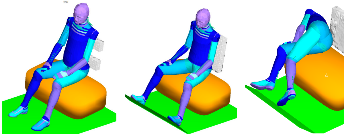
Figure 1. Human model in the vibration test on an experimental seat with a configurable backrest and two foam blocks modelled using finite elements (left) and on the rear bench of a Prius vehicle in the slalom test (middle) and falling without leg control in the slalom (right).
