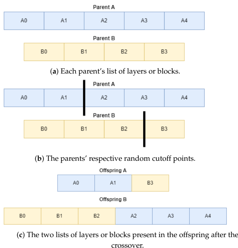
Figure 2. Visualization of the one-point crossover on a list of convolutional blocks or dense layers in a NASCTY genome.
