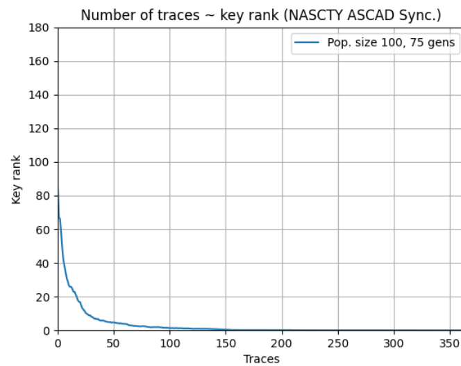
(a) The mean performance of the best neural network over 100 folds.
