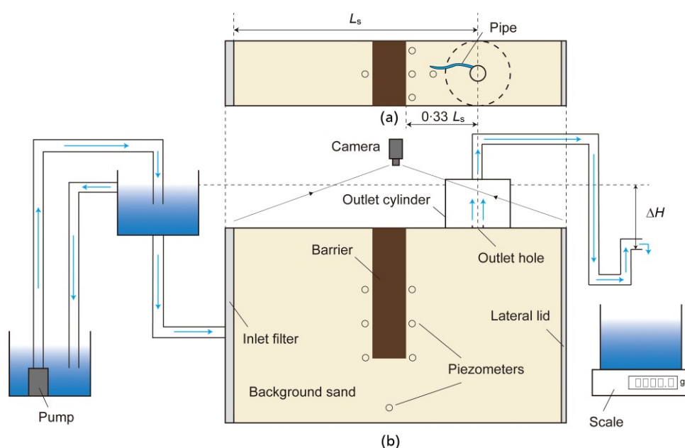
Fig. 3. Scheme of the experimental set-up of BEP tests: (a) plan (top) view and (b) front view. L_s is the distance from the inlet to the outlet
