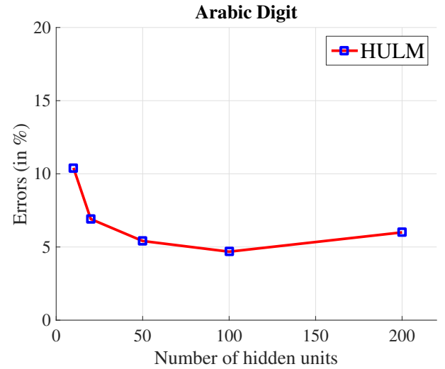
Fig. 6: Generalization error (in %) of the hidden-unit logistic model on the Arabic speech data set as a function of the number of hidden units.
