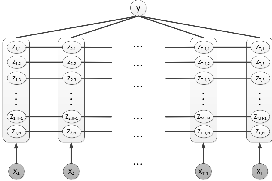
Fig. 1: Graphical model of the hidden-unit logistic model.
