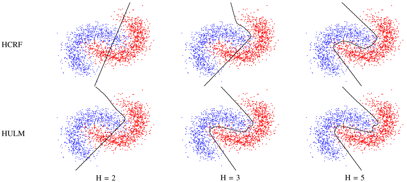
Fig. 3: Comparison of HCRF and HULM for binary classification on the banana dataset (ignoring the time series aspect of the models) with the same number of hidden units H . The black lines show the decision boundaries learned by both models.
