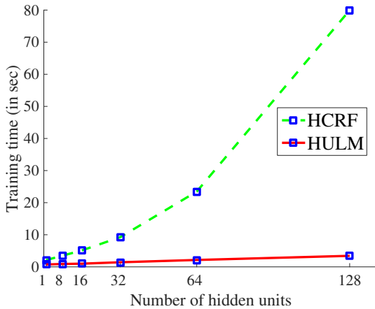
Fig. 4: Running time of a single training epoch of the HULM and HCRF model on the facial expression data (CK+) described in Sec. IV-A as a function of the number of hidden units. We used stochastic gradient descent with the same configuration to train both the HULM and the HCRF.
