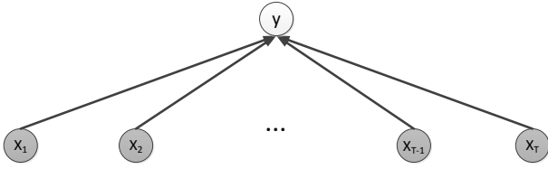
Fig. 5: Graphical model of the naive logistic model.
