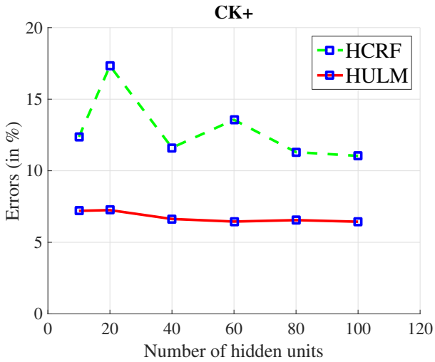
Fig. 7: Generalization error (in %) of the hidden-unit logistic model and the hidden CRF on the CK+ data set as a function of the number of hidden units.
