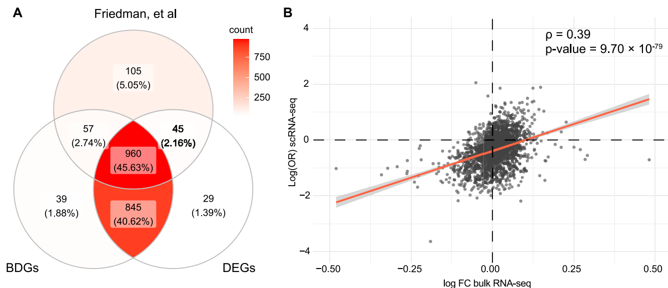
Figure 2. (A) Venn diagram of genes detected ( P_{\text{FDR}} \leq 0.05 ) in a bulk AD dataset (Friedman et al. ), in the single cell AD dataset with BDA-LR (BDGs) and with DEA (DEGs). Each section shows the number and percentage of genes belonging to that section. (B) Plot of the \log(\text{FC}) from the AD bulk dataset (x-axis) and the \log(\text{OR}) from the single cell AD dataset (y-axis). The red line represents the linear association between the bulk \log(\text{FC}) and \log(\text{OR}) . The Spearman's rank correlation coefficient ( \rho ) and corresponding association P -value are also shown. Outlier genes ( n = 9 , B) were removed from the plots.
