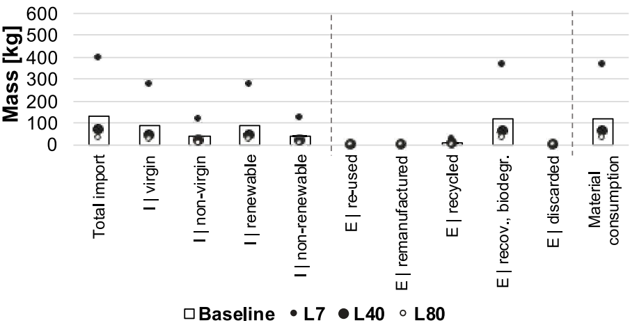
Figure A.H2a. MFA Sensitivity analysis on the L_{\text{technical}} and L_{\text{functional}} for the BAU kitchen (material flows over 80 years)
