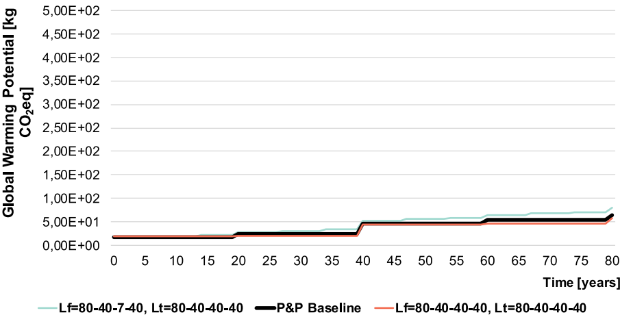
Figure A.H1g. LCA Sensitivity analysis on the L_{\text{functional}} for the P&P kitchen (GWP allocated over 80 years)
