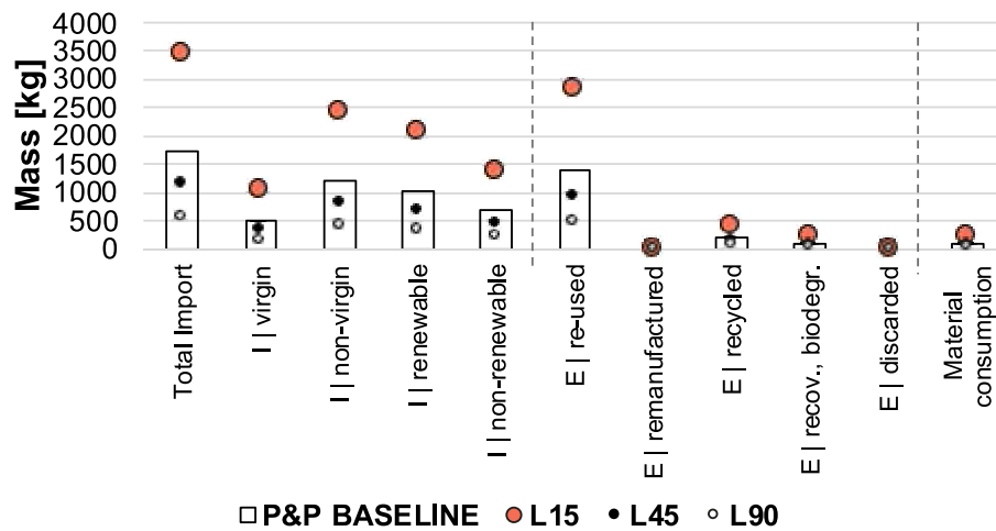
Figure A.12e. MFA Sensitivity analysis on the L_{\text{technical}} and L_{\text{functional}} for the P&P façade (material flows over 90 years)
