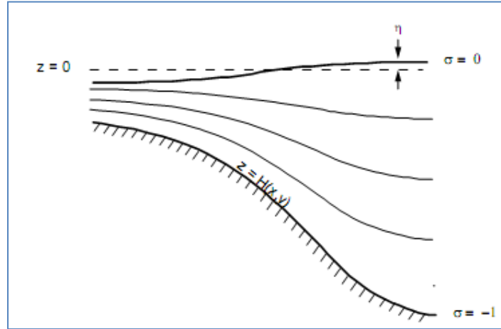
Figure 2.7: Typical sigma coordinate (Mellor, 2004)
