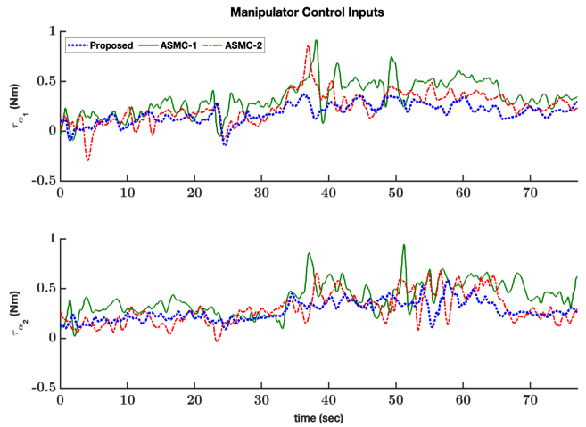
Fig. 7. Comparison of manipulator control inputs with various controllers.
