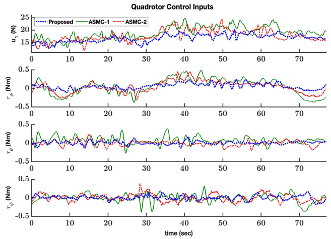
Fig. 6. Comparison of quadrotor control inputs with various controllers.
