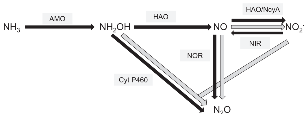
Fig. 3. Putative \text{N}_2\text{O} emission pathways in AOB. Black arrows represent biologically mediated pathways, grey arrows represent abiotic conversions. AMO – ammonium monooxygenase, HAO – hydroxylamine oxidoreductase, NcyA – Nitrososcyanin, Cyt P460 – Cytochrome P460, NIR – nitrite reductase, NOR – NO reductase. Sources: Caranto et al., 2016; Soler-Jofra et al., 2018; Stein 2019; Terada et al., 2017.
