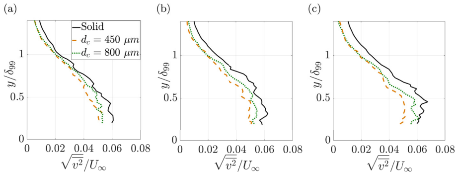
Fig. 16. R.m.s. wall-normal velocity \sqrt{v^2}/U_\infty at three different streamwise locations: x/c = -0.08 (a), x/c = -0.05 (b) and x/c = -0.02 (c).
