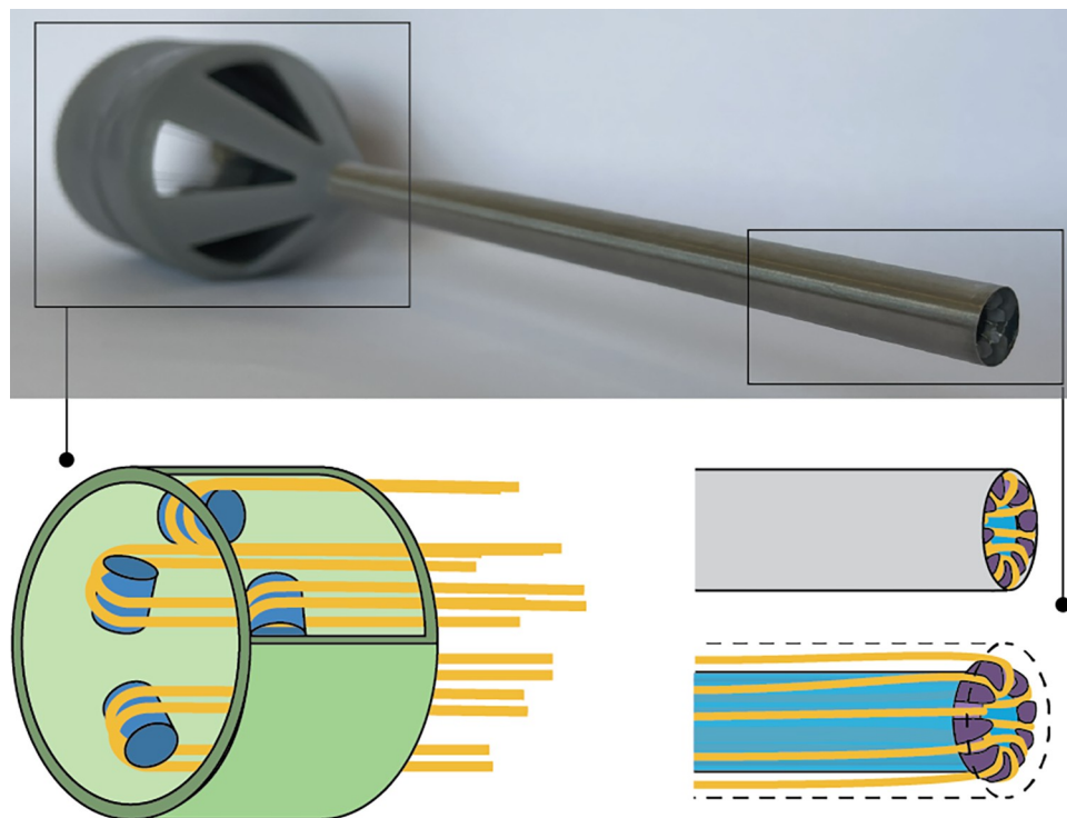
Fig 3. Schematic view of the actuation side of the device and the distal end of the cone. Viewed with and without the outer tube.
